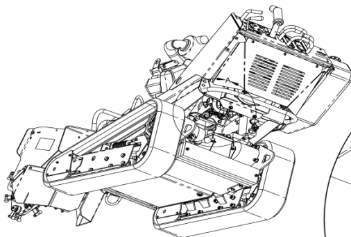
BYPASS VALVES (2 HEX PLUGS WITH CROSS HOLE) LOOSEN 2 TURNS TO TOW DISABLED MACHINE ONTO TRAILER
