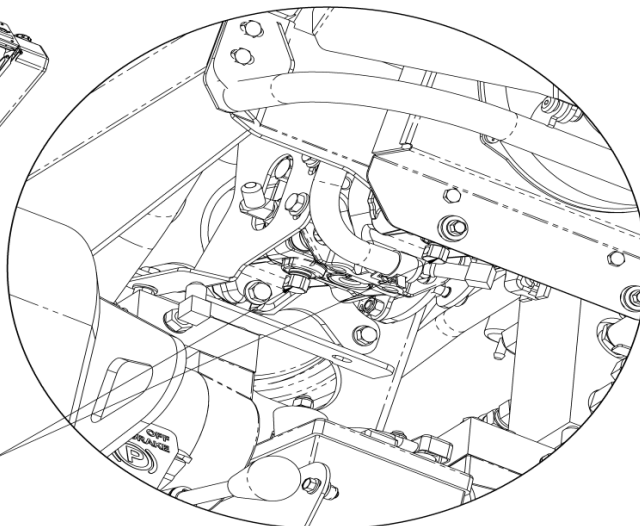
BYPASS VALVES (2 HEX PLUGS WITH CROSS HOLE) LOOSEN 2 TURNS TO TOW DISABLED MACHINE ONTO TRAILER
